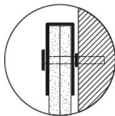
Wall Mounted
